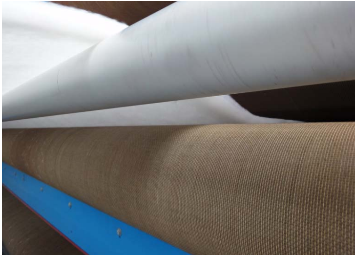
Picture 1: Anti-stick coated glass hybrid belts for use in single-belt and double-belt dryers combine low weight with transverse stability thanks to its use of glass strands that are interwoven in the running direction.
